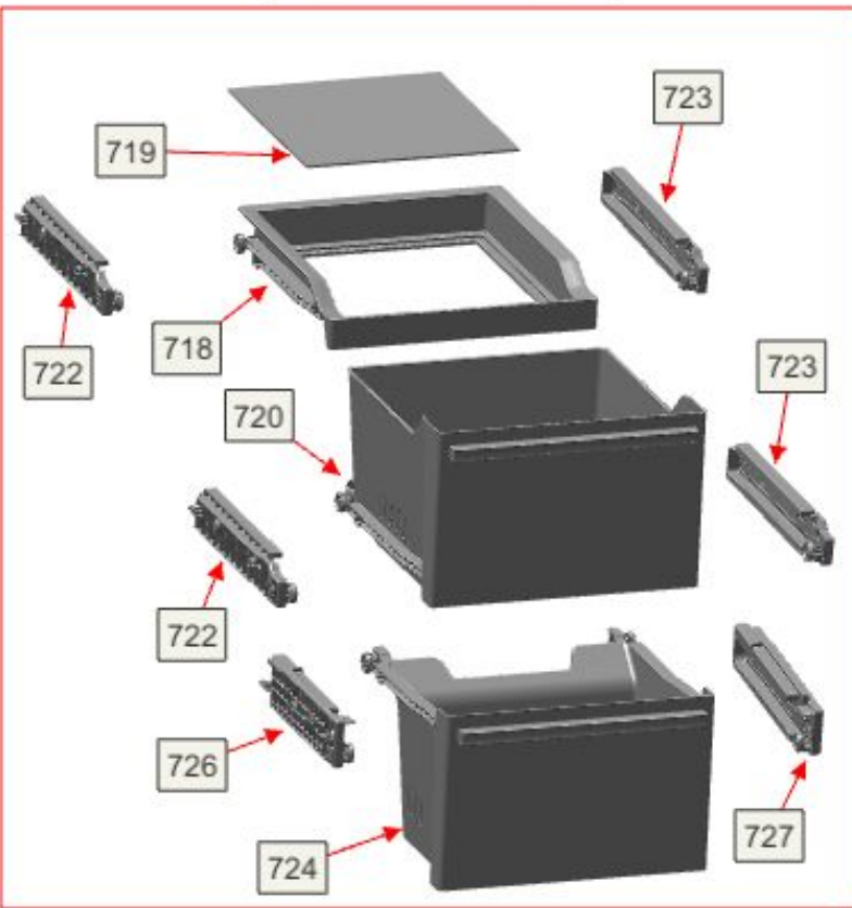
Compartimento Freezer
